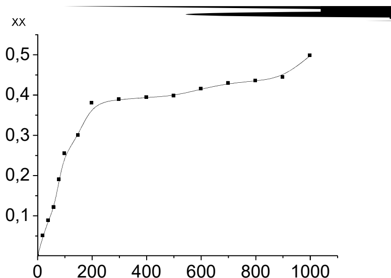
4-rasm. Salt yurish kuchlanishining yoritilganlik intensivligiga bog'liqligi
